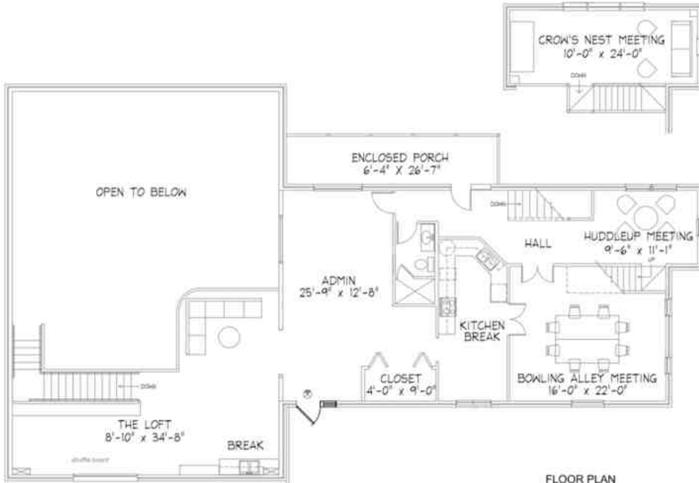
FLOOR PLAN 2ND FLOOR 1212 6TH AVE N. NASHVILLE, TN 37208
