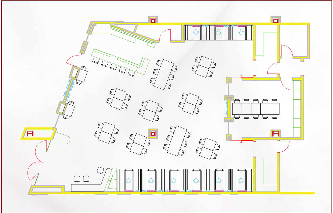
Cin City Layout—40 seats
