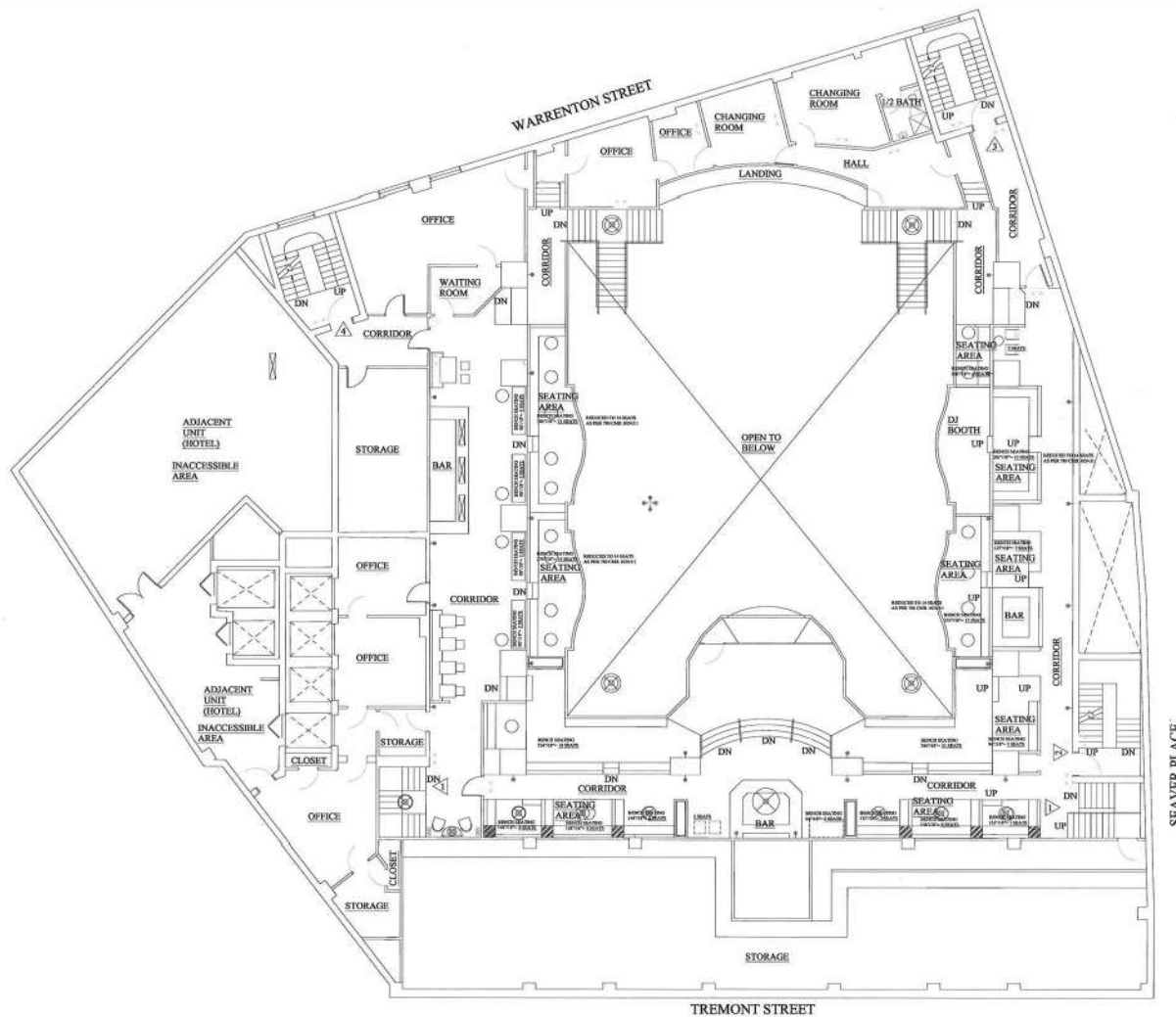
MEZZ. FLOOR PLAN
