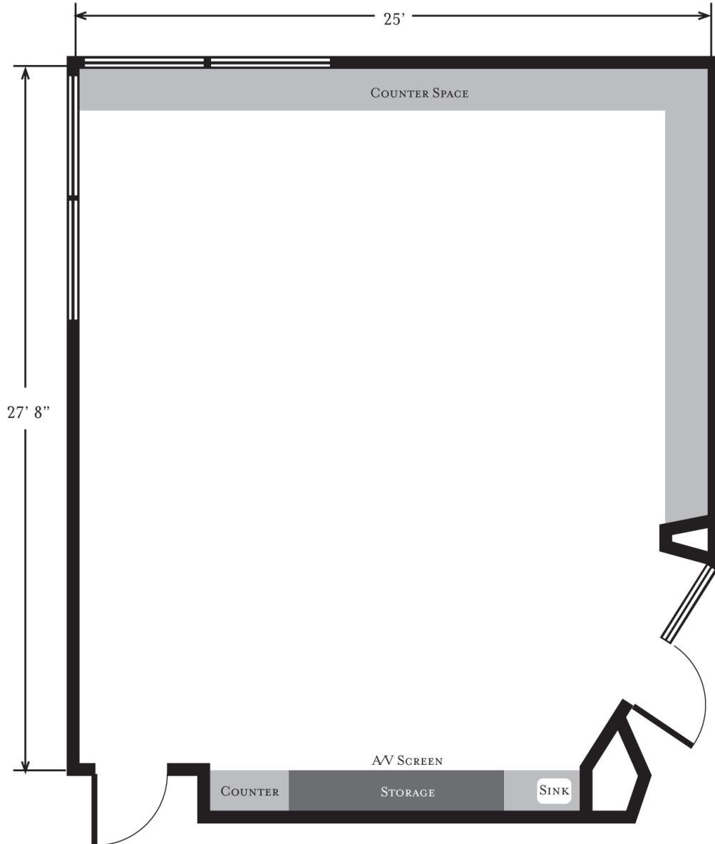
Tamátslikt Classroom CEILING HEIGHT: 10' - 12' SCALE: 3/16"=1' 694 SQ. FT.
